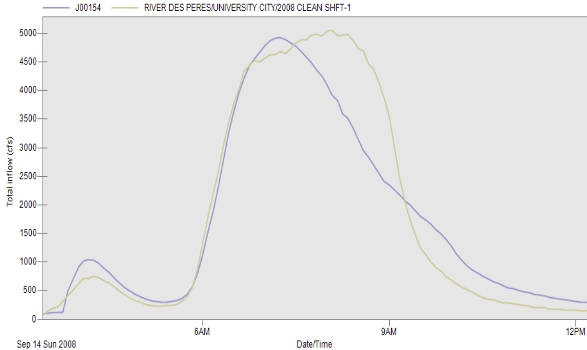
Figure 4. PCSWMM September 2008 verification results
