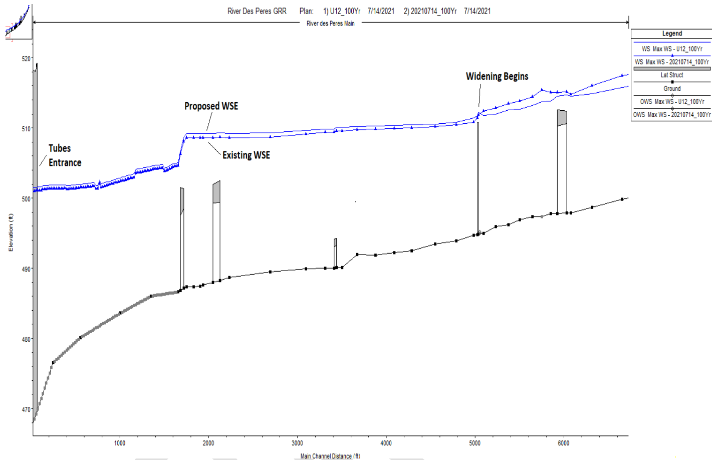
Figure 26. Original TSP, Alternative U12, Channel Widening - 1% AEP Water Surface Profile
