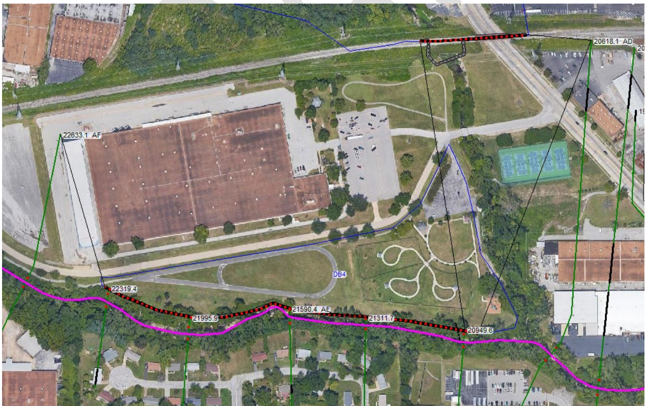
Figure 18. HEC-RAS Detention Basin 4 Configuration
