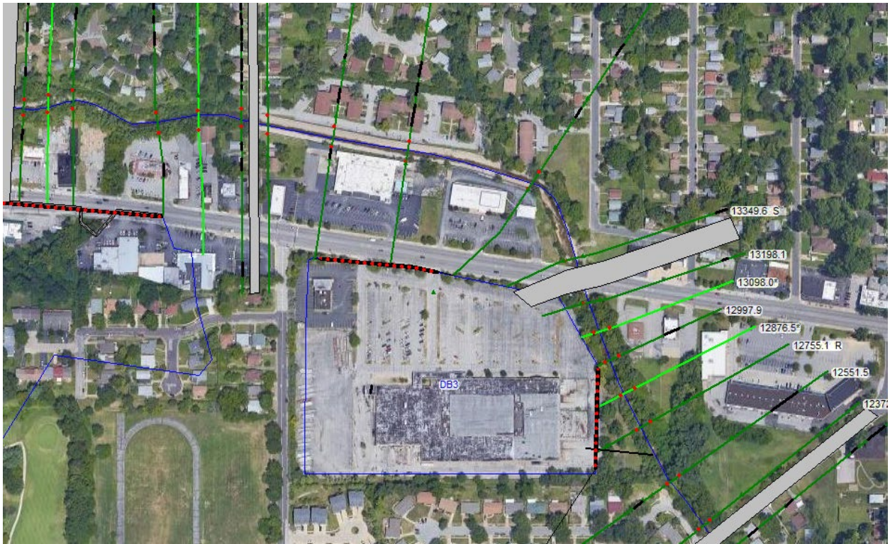
Figure 17. HEC-RAS Detention Basin 3 Configuration
