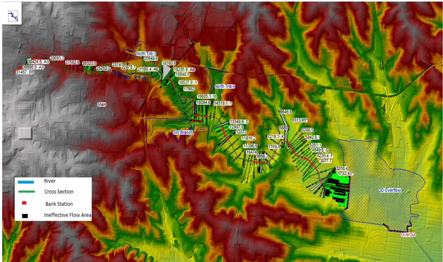
Figure 2 - HEC-RAS Model of the University City Branch of the River Des Peres
