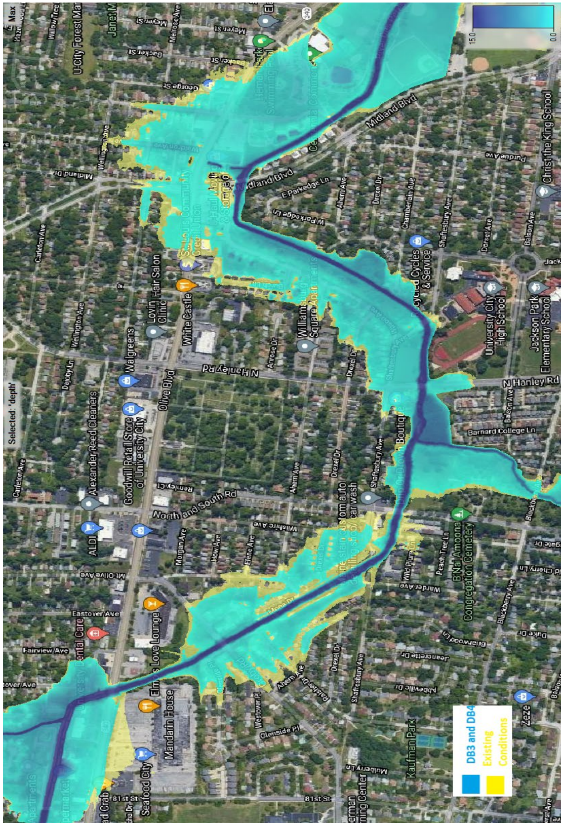
Figure 22. Proposed DB3 and 4 Alternative versus Existing Conditions Inundation - 1% AEP - Groby/Shafsbury/Wilson Vicinity
