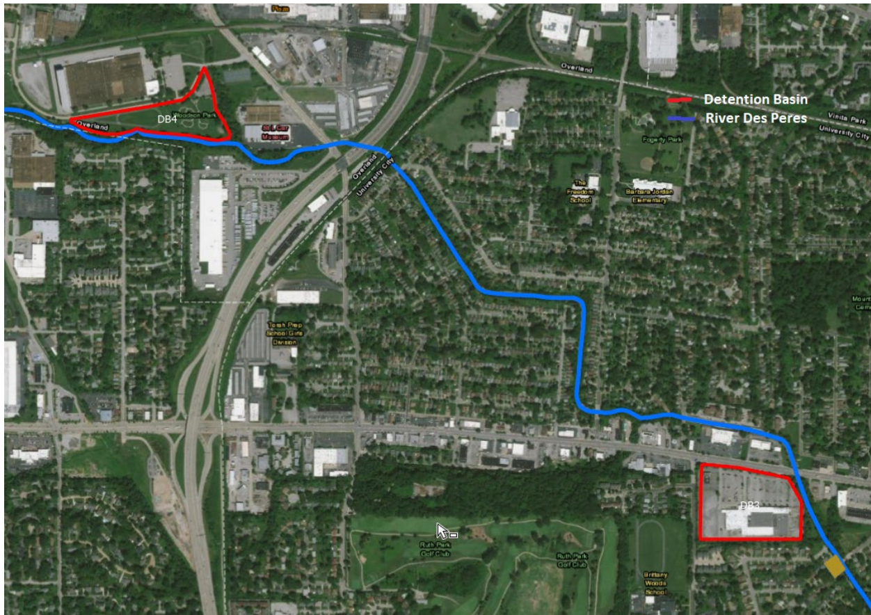
Figure 16. Location of Detention Basins 3 and 4 (retained)
