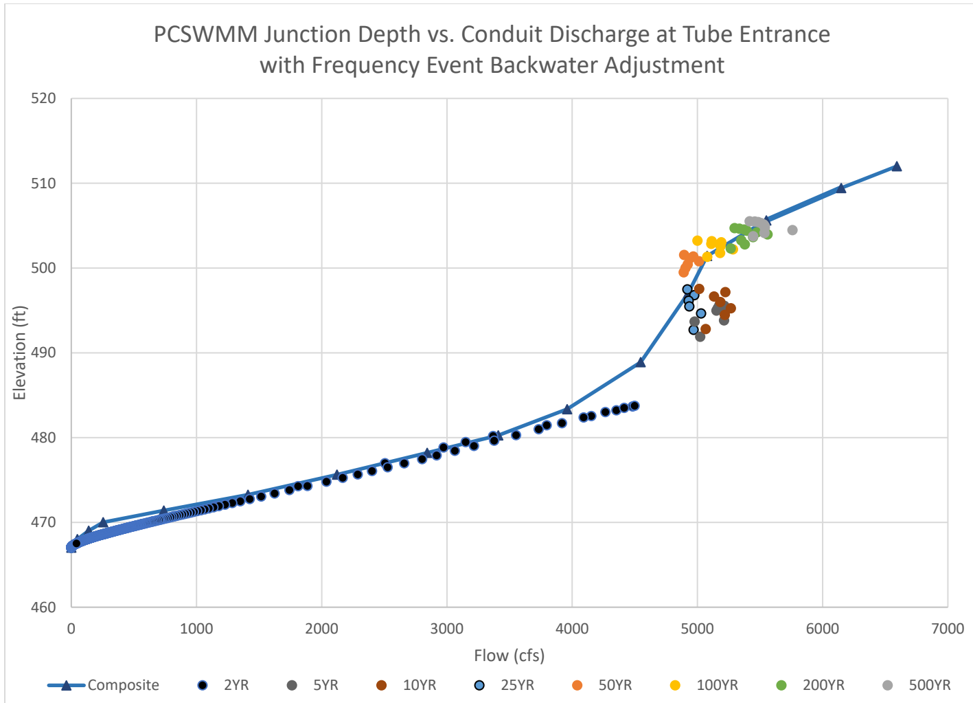
Figure 6 - Adjusted Rating Curve at Tube Entrance Accounting for Backwater Influence
