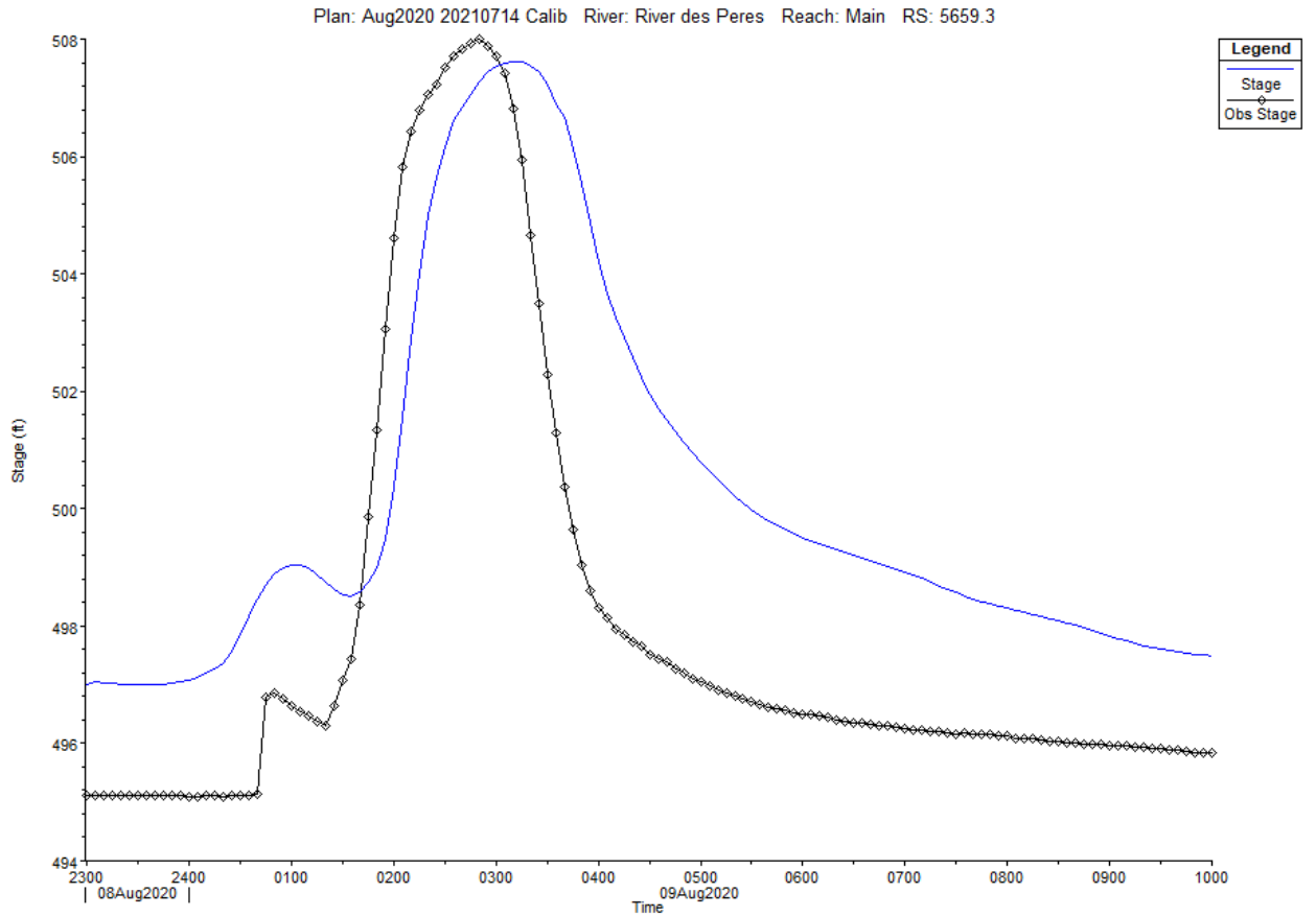
Figure 7. Computed versus observed water surface at River Des Peres, University City gage August 2020
