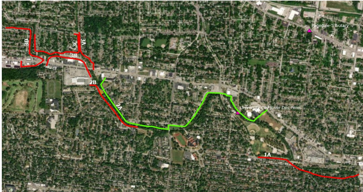
Figure 25. Proposed Levee Alignments
