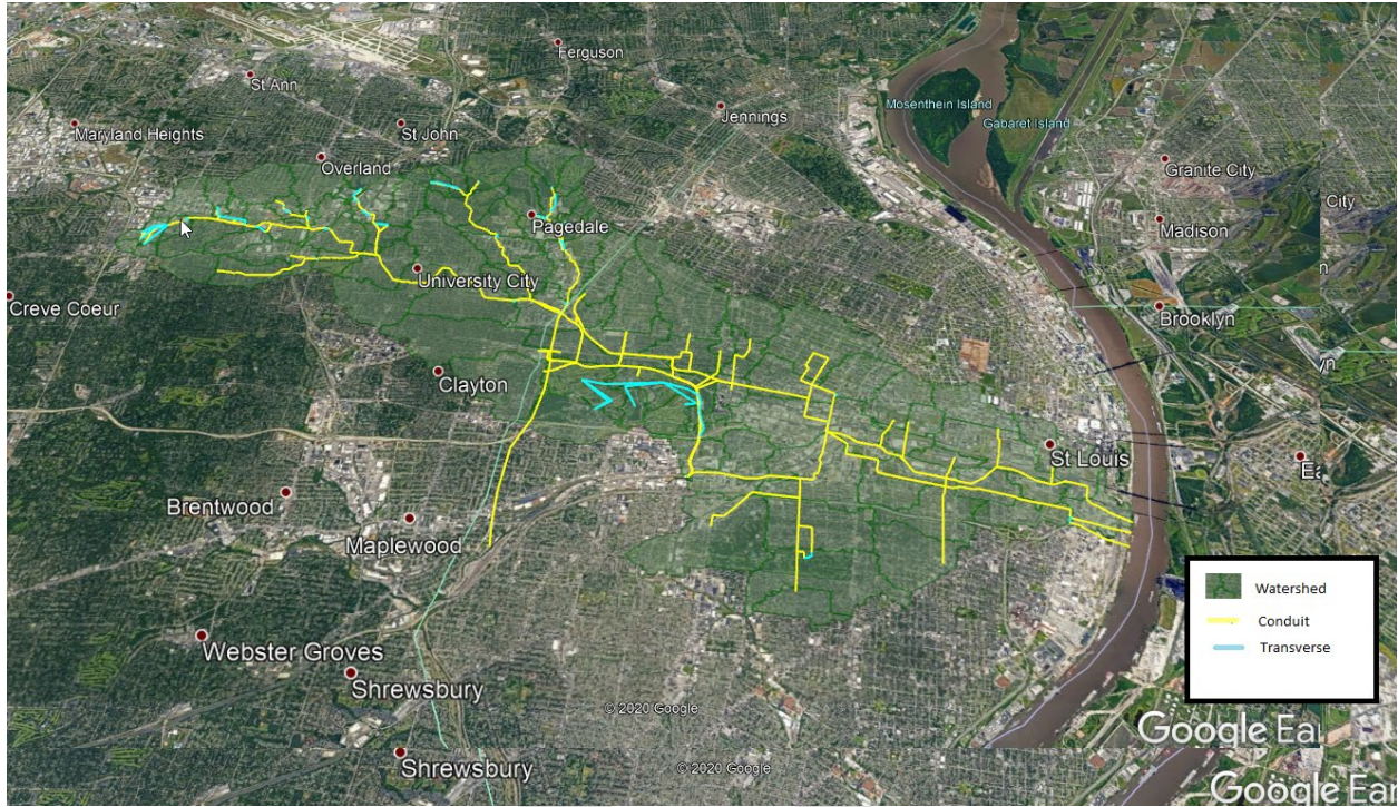
Figure 1 - PCSWMM Geometry of the Upper River Des Peres Watershed
