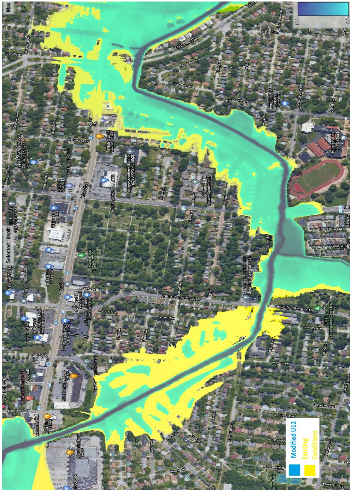
Figure 28. Proposed Modification to U12 Alternative versus Existing Conditions Inundation - 1% AEP - Groby/Shafsbury/Wilson Vicinity
