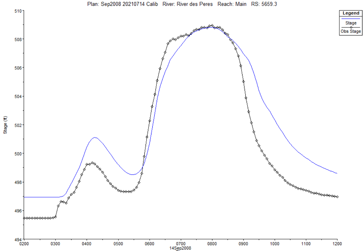
Figure 8. Computed versus observed water surface at River Des Peres, University City gage September 2008
