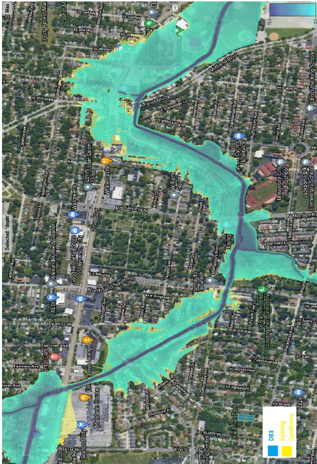
Figure 23. Proposed DB3 Alternative versus Existing Conditions Inundation - 1% AEP - Groby/Shafsbury/Wilson Vicinity
