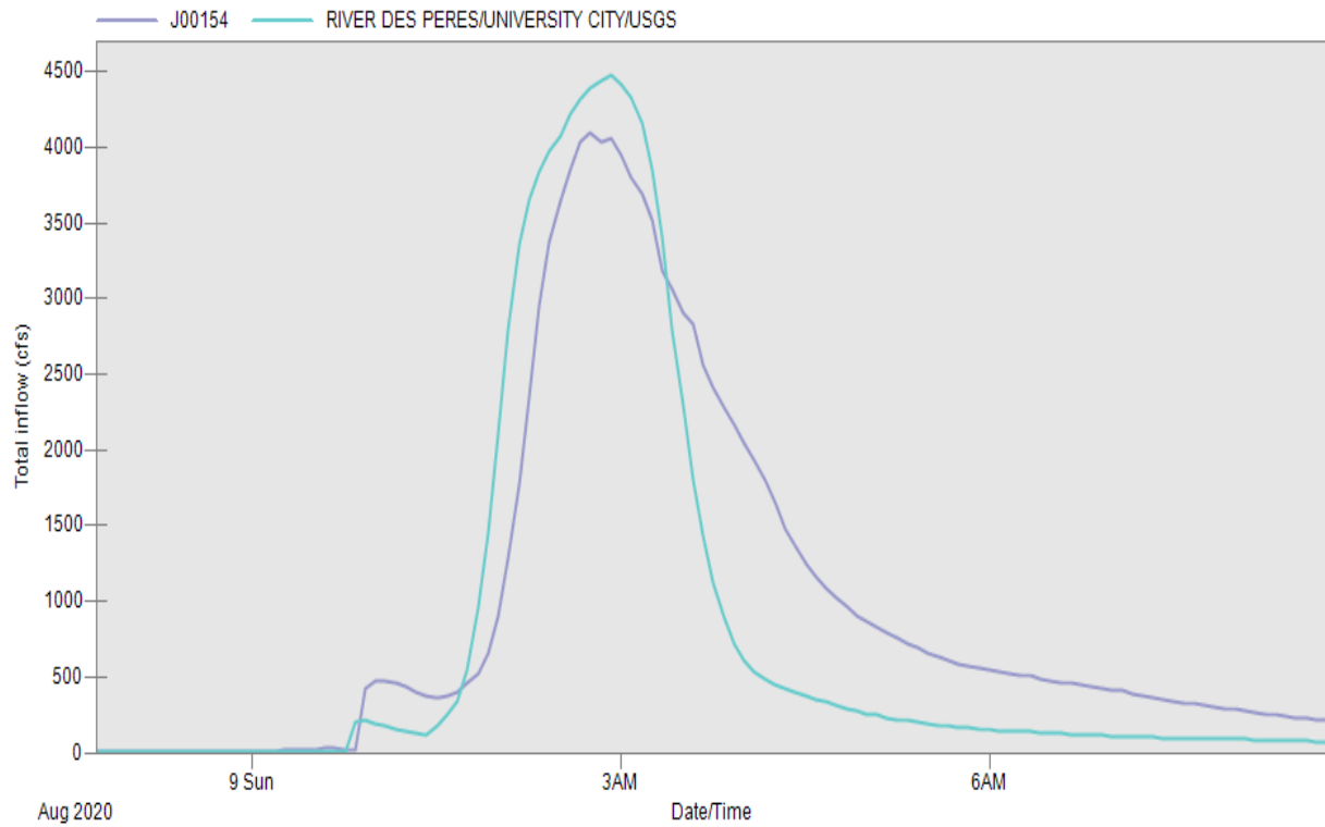
Figure 3. PCSWMM August 2020 calibration results
