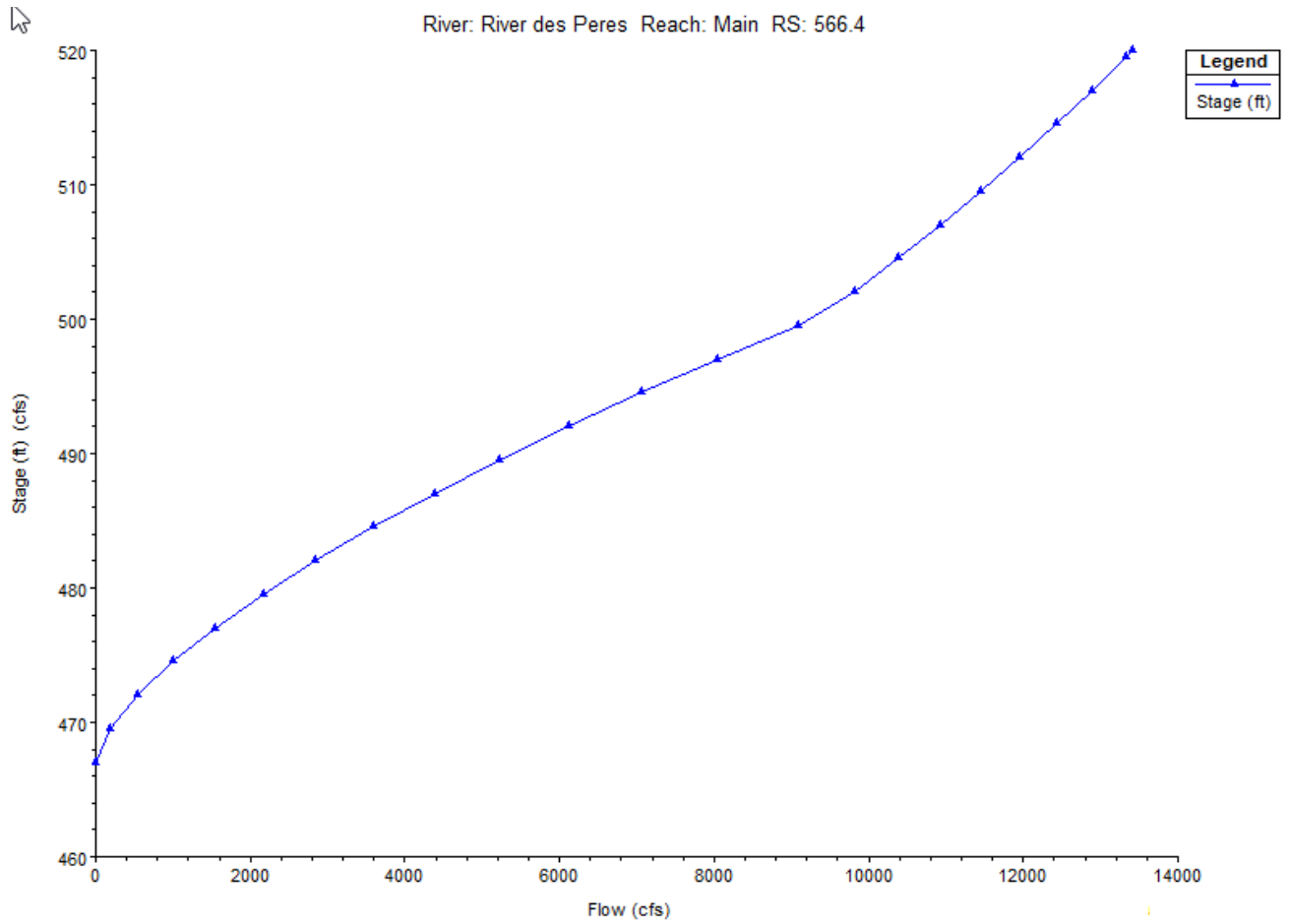
Figure 5. Downstream culvert Boundary Rating Curve Without Backwater Adjustment
